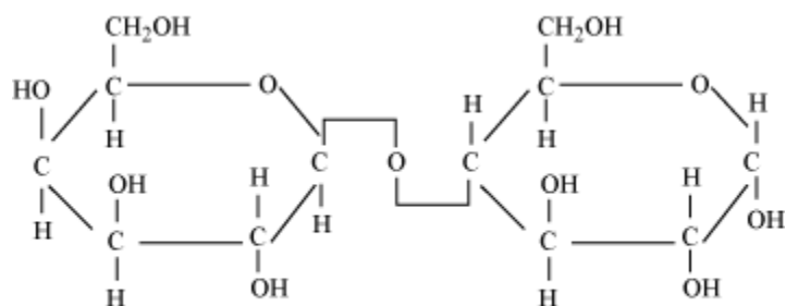
Glycosidic bond
